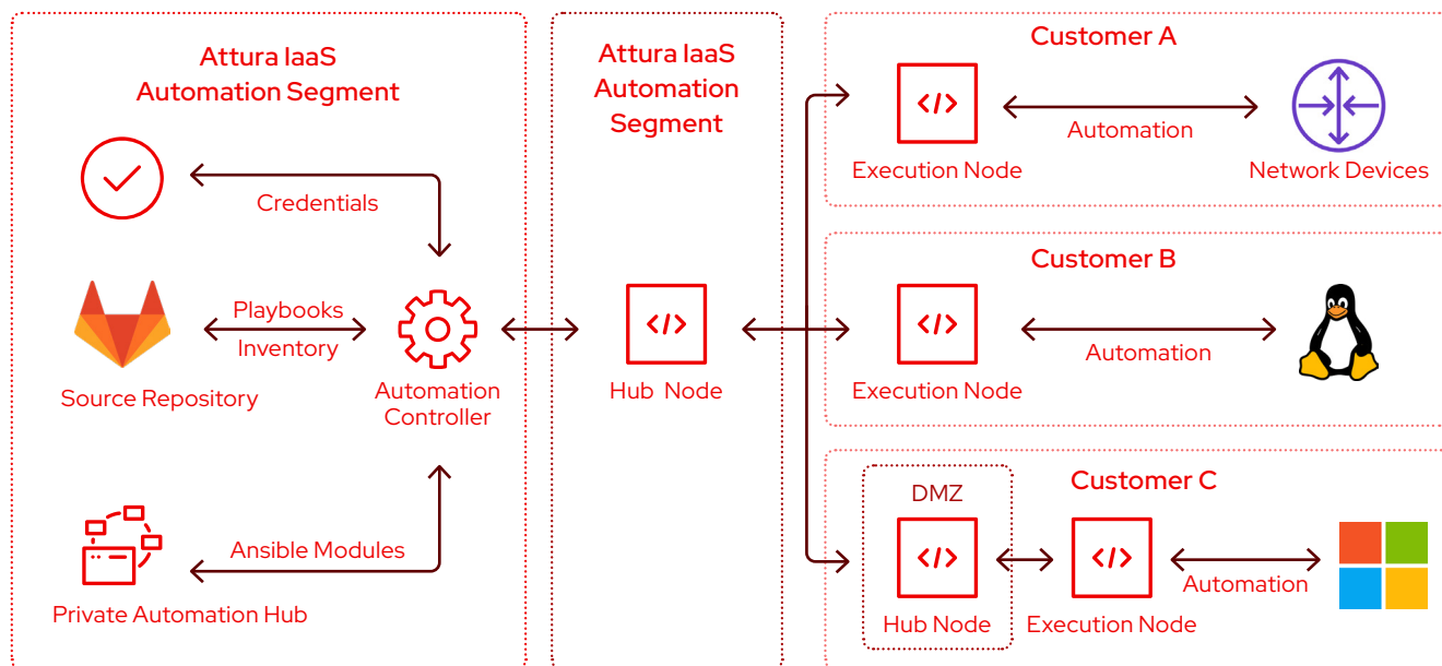
Figure 1: System architecture
